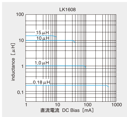
直流重畳特性例 DC Bias characteristics (Measured by HP4194A)
