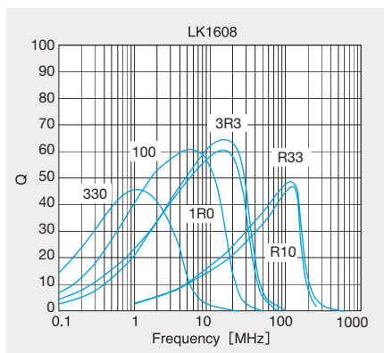
Q-周波数特性例 Q-vs-Frequency characteristics (Measured by HP4294A or HP4291A)
